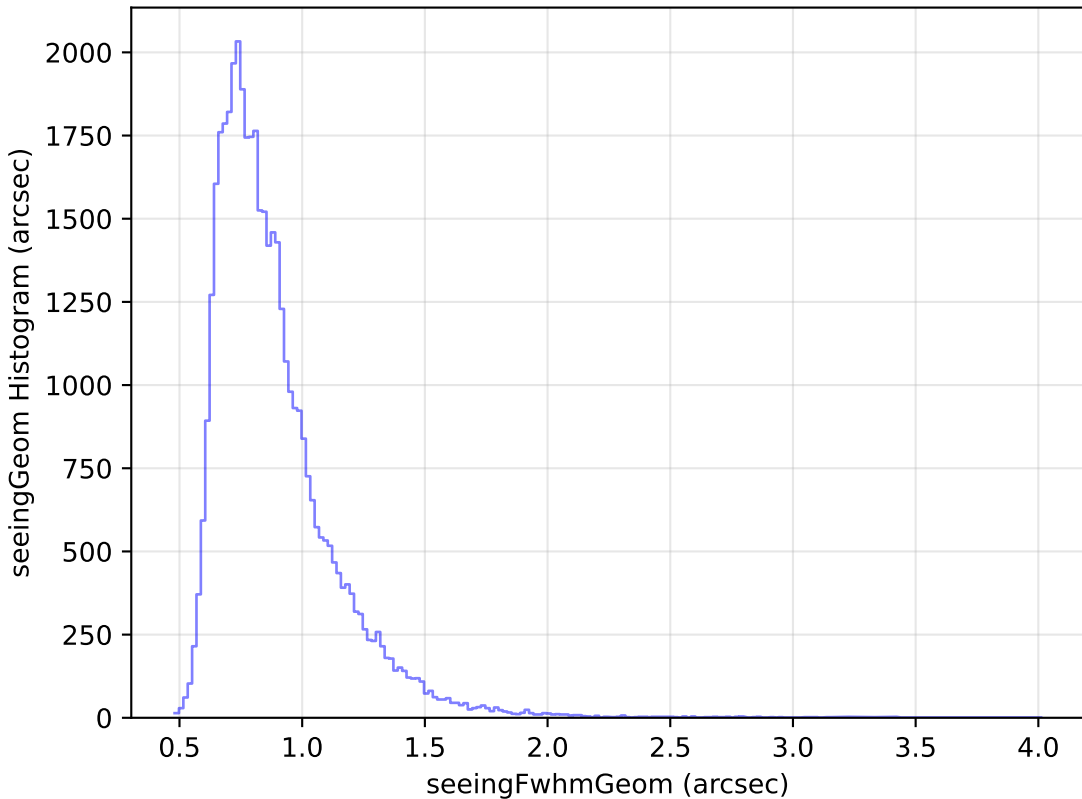
weather_cloudso4v3.4_10yrs Yr 1 z band: seeingGeom Histogram
