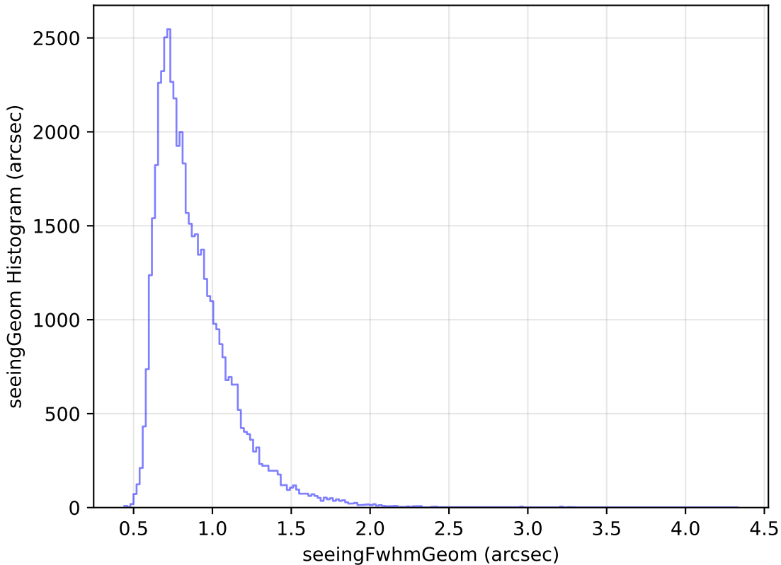
weather_cloudso4v3.4_10yrs Yr 1 r band: seeingGeom Histogram
