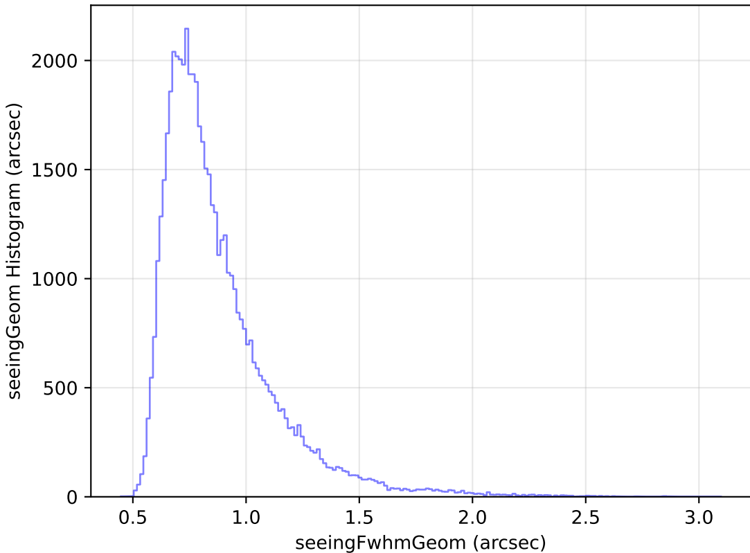
weather_cloudso4v3.4_10yrs Yr 1 i band: seeingGeom Histogram
