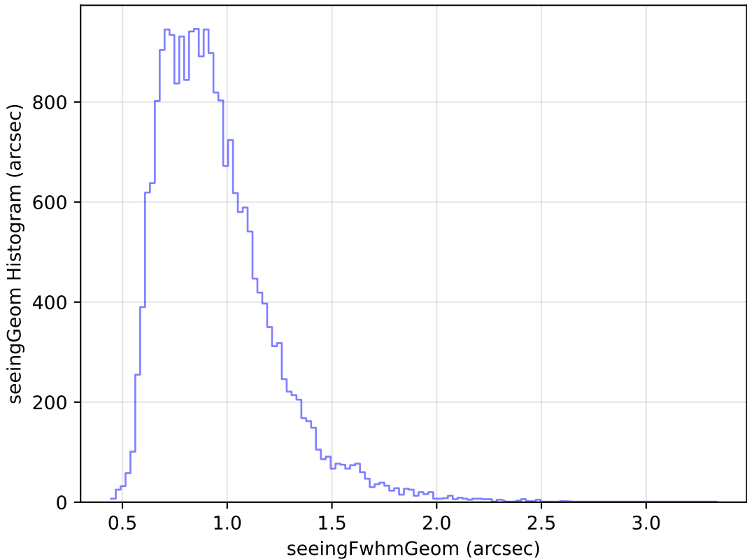
weather_cloudso4v3.4_10yrs Yr 1 g band: seeingGeom Histogram
