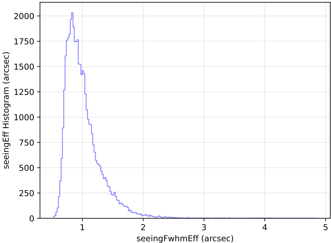
weather_cloudso4v3.4_10yrs Yr 1 z band: seeingEff Histogram
