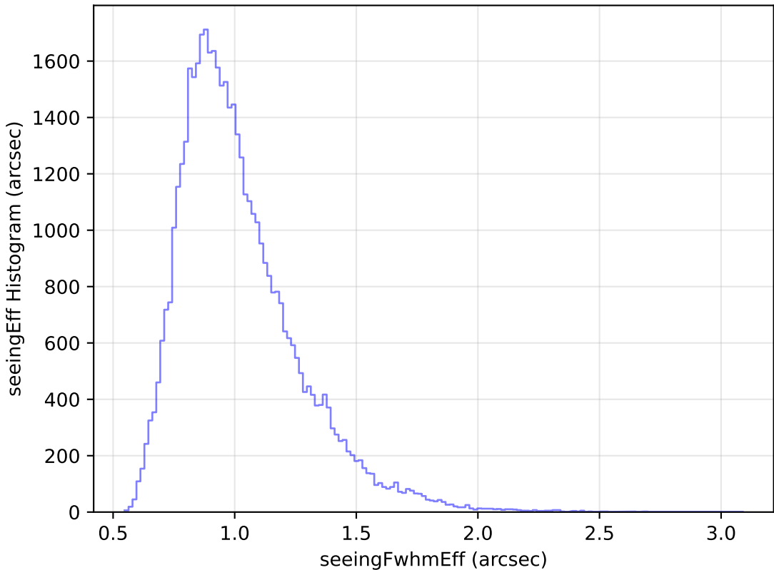
weather_cloudso4v3.4_10yrs Yr 1 y band: seeingEff Histogram
