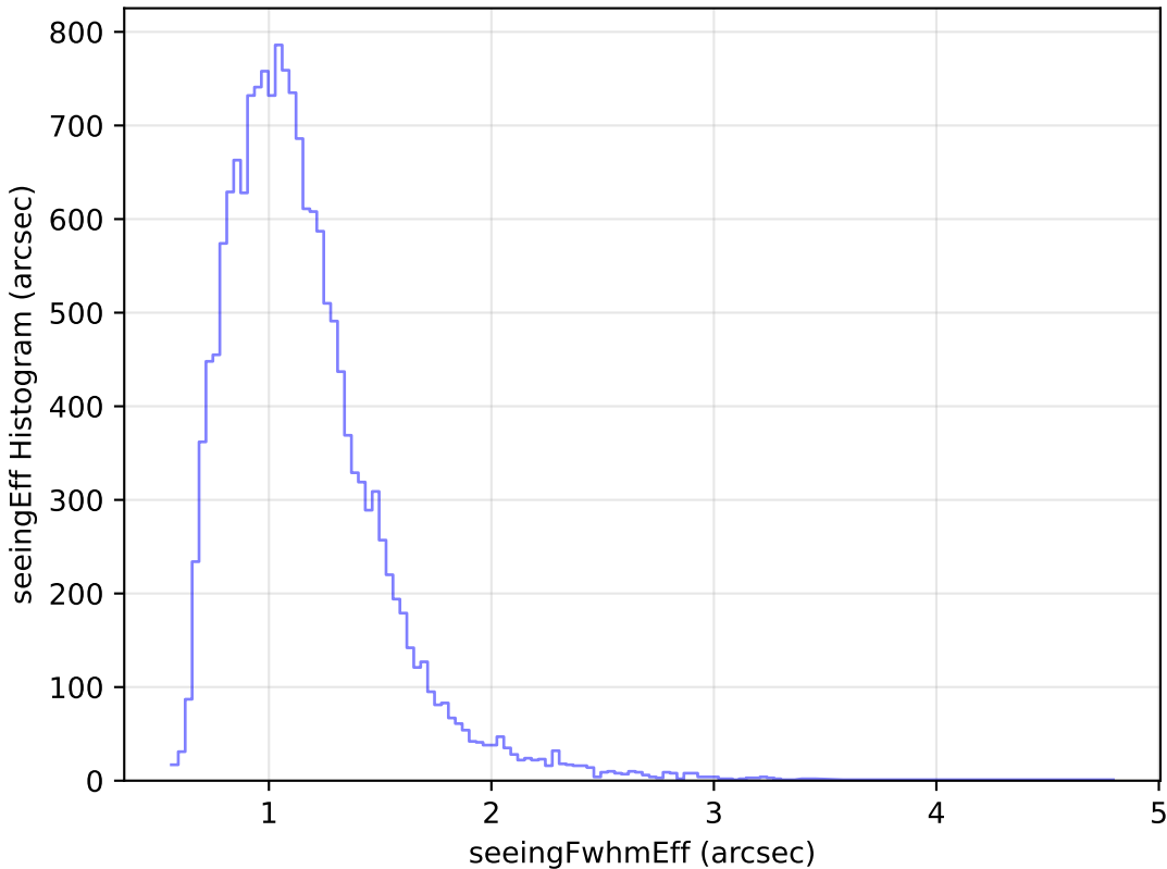
weather_cloudso4v3.4_10yrs Yr 1 u band: seeingEff Histogram
