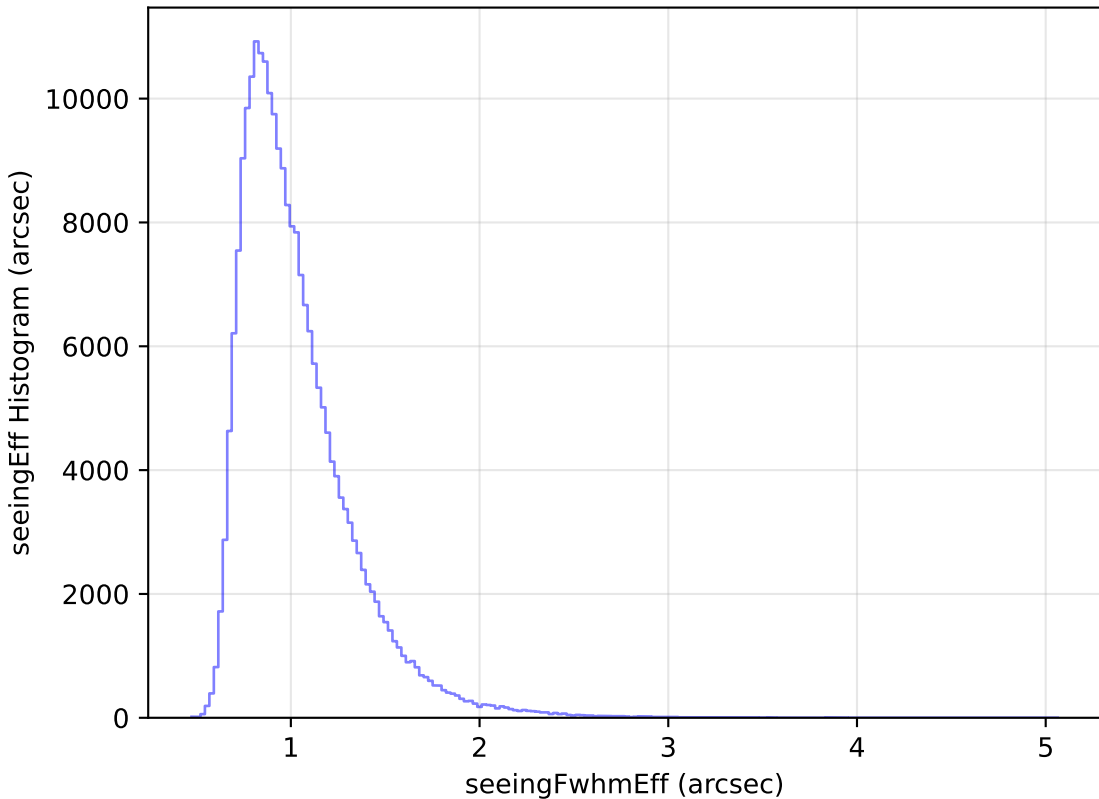
weather_cloudso4v3.4_10yrs Yr 1 all bands: seeingEff Histogram
