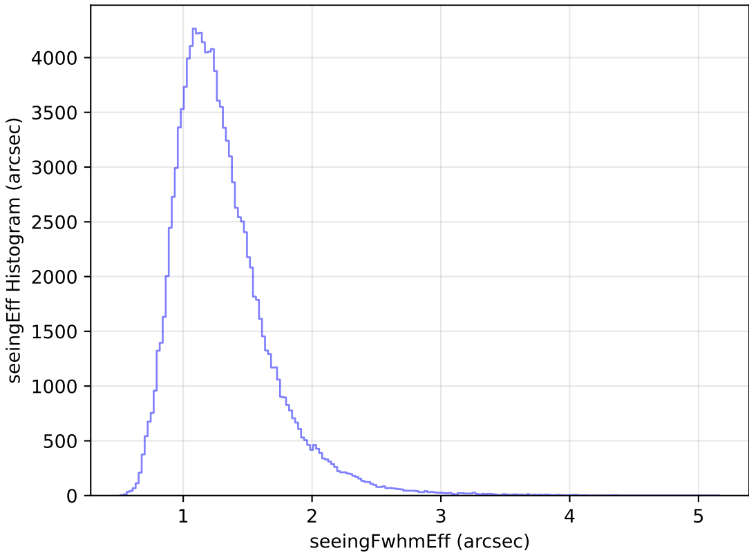
weather_cloudso4v3.4_10yrs WFD u band: seeingEff Histogram
