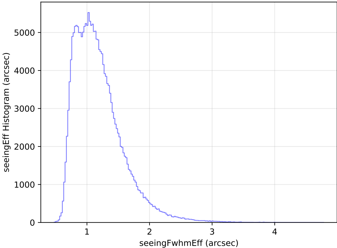
weather_cloudso4v3.4_10yrs WFD g band: seeingEff Histogram
