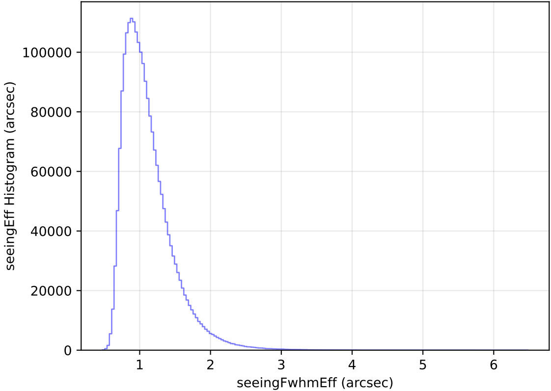
weather_cloudso4v3.4_10yrs WFD all bands: seeingEff Histogram
