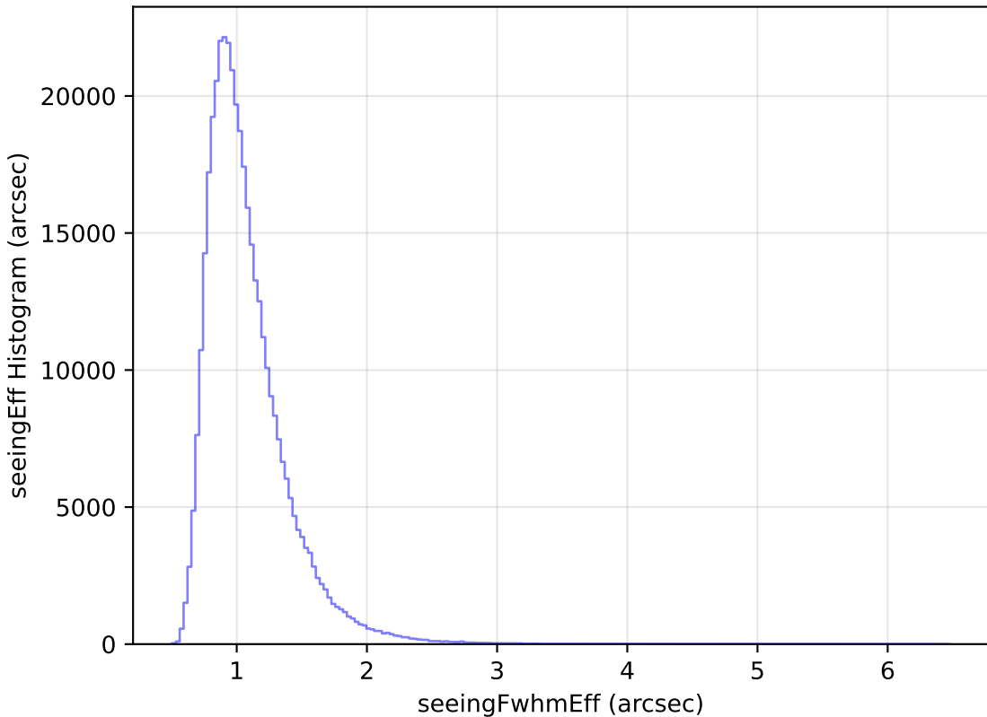
weather_cloudso4v3.4_10yrs All sky y band: seeingEff Histogram
