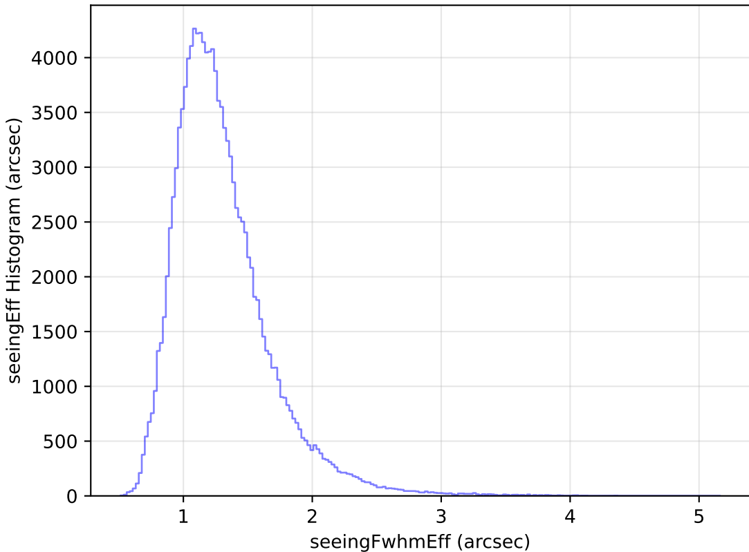
weather_cloudso4v3.4_10yrs All sky u band: seeingEff Histogram
