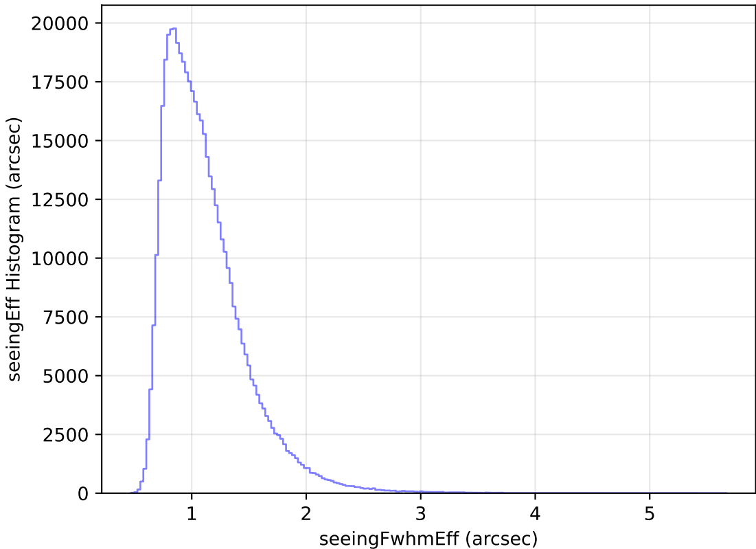
weather_cloudso4v3.4_10yrs All sky r band: seeingEff Histogram
