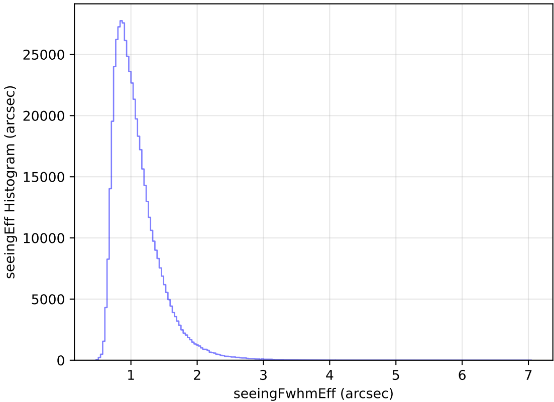
weather_cloudso4v3.4_10yrs All sky i band: seeingEff Histogram
