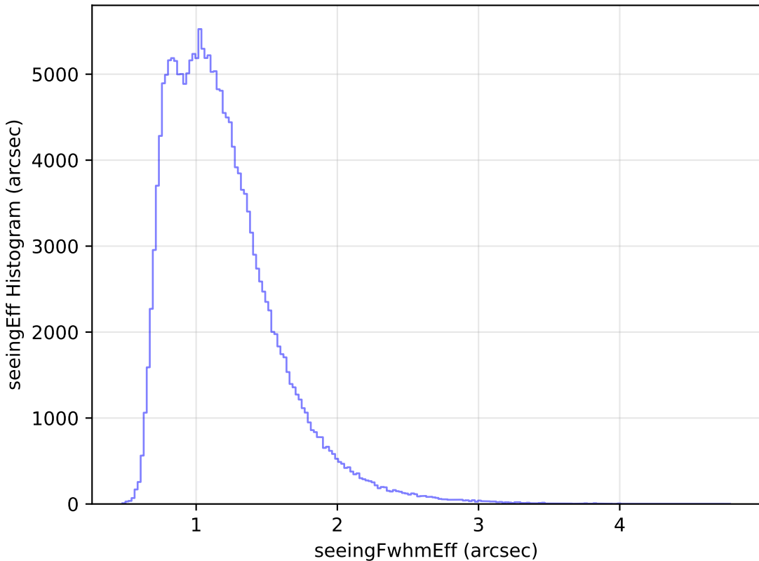
weather_cloudso4v3.4_10yrs All sky g band: seeingEff Histogram
