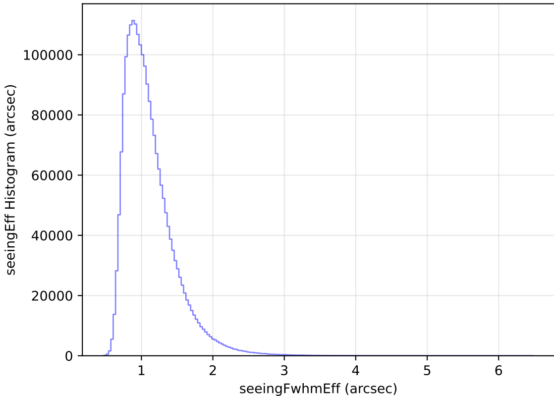
weather_cloudso4v3.4_10yrs All sky all bands: seeingEff Histogram
