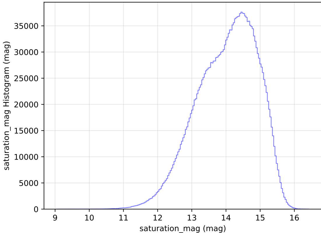
weather_cloudso4v3.4_10yrs All sky all bands: saturation_mag Histogram
