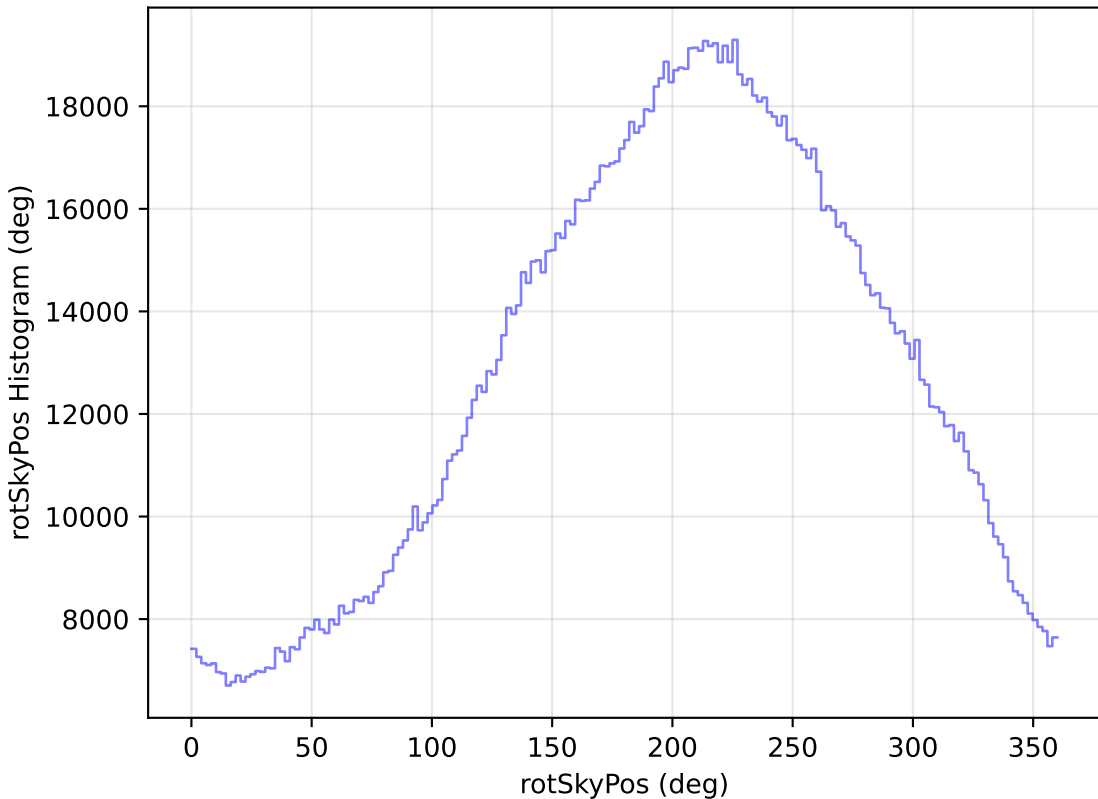
weather_cloudso4v3.4_10yrs WFD all bands: rotSkyPos Histogram
