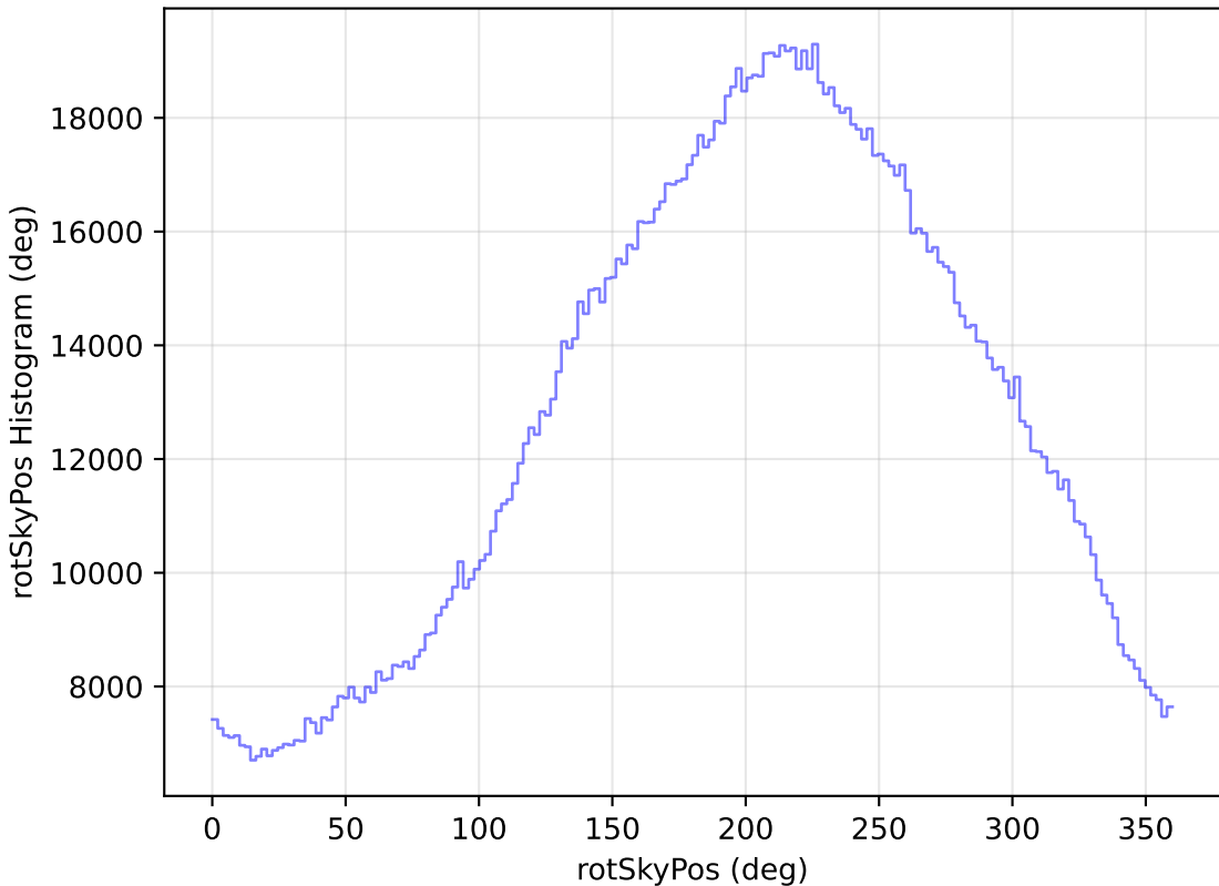
weather_cloudso4v3.4_10yrs All sky all bands: rotSkyPos Histogram
