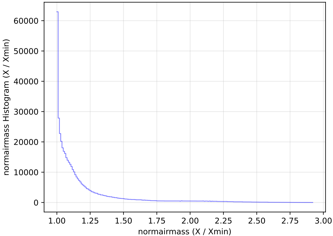
weather_cloudso4v3.4_10yrs WFD z band: normairmass Histogram
