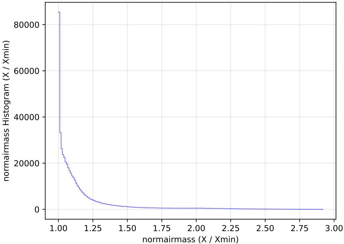
weather_cloudso4v3.4_10yrs WFD i band: normairmass Histogram
