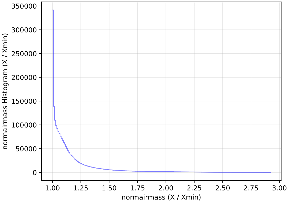
weather_cloudso4v3.4_10yrs WFD all bands: normairmass Histogram
