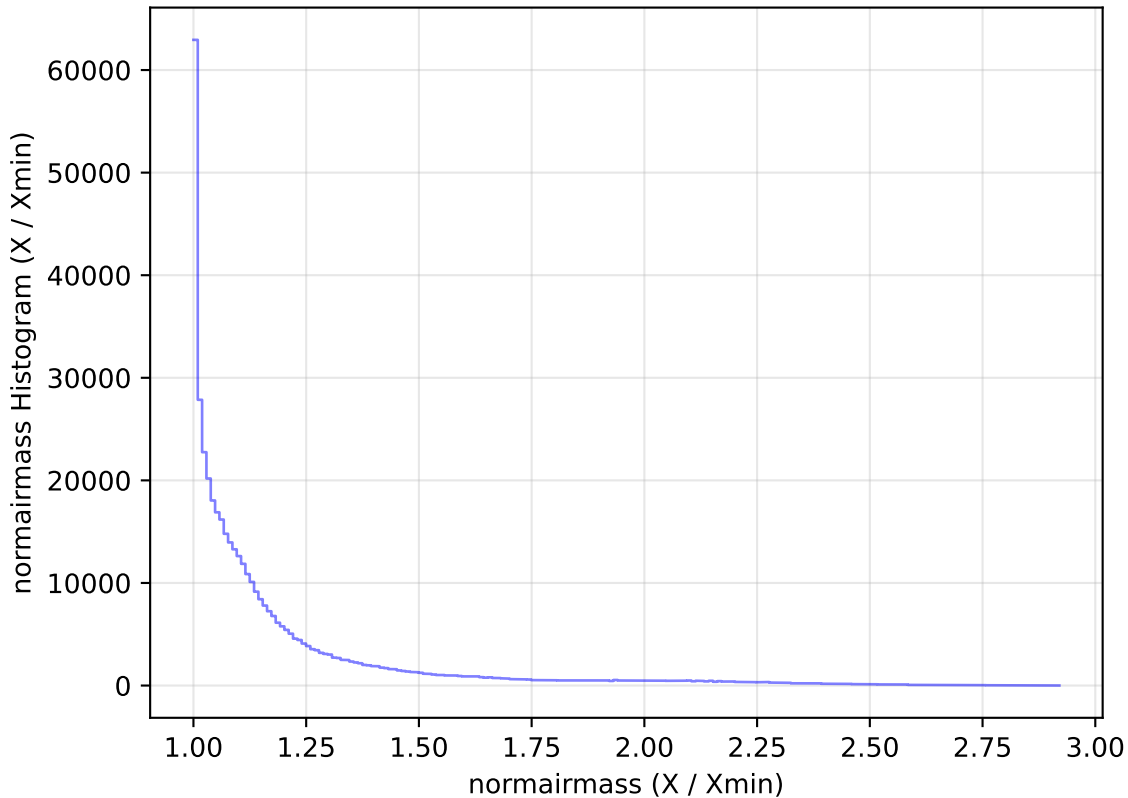
weather_cloudso4v3.4_10yrs All sky z band: normairmass Histogram
