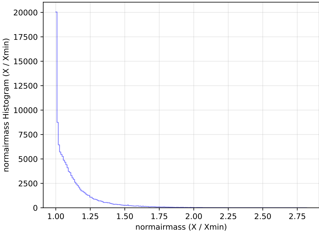
weather_cloudso4v3.4_10yrs All sky u band: normairmass Histogram
