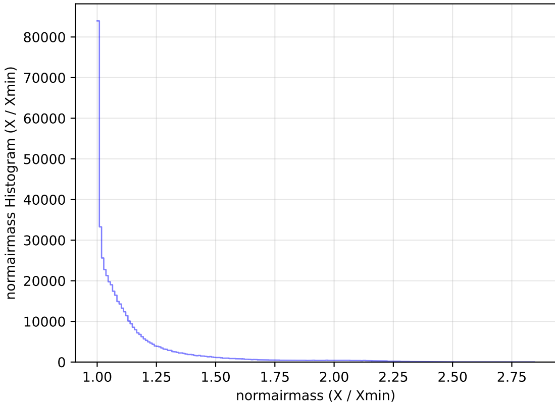
weather_cloudso4v3.4_10yrs All sky r band: normairmass Histogram
