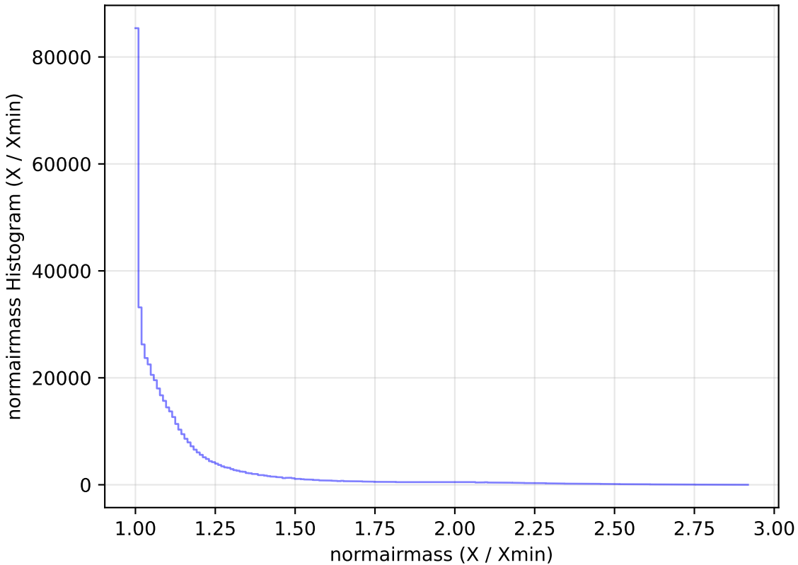
weather_cloudso4v3.4_10yrs All sky i band: normairmass Histogram
