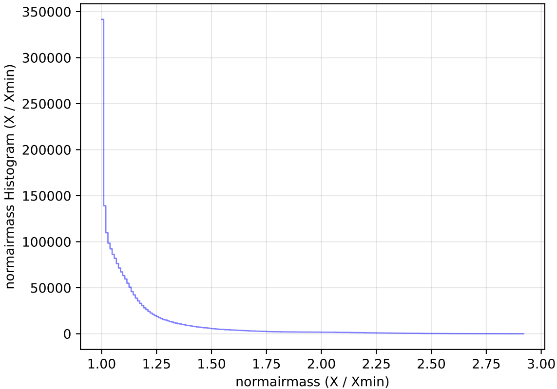
weather_cloudso4v3.4_10yrs All sky all bands: normairmass Histogram
