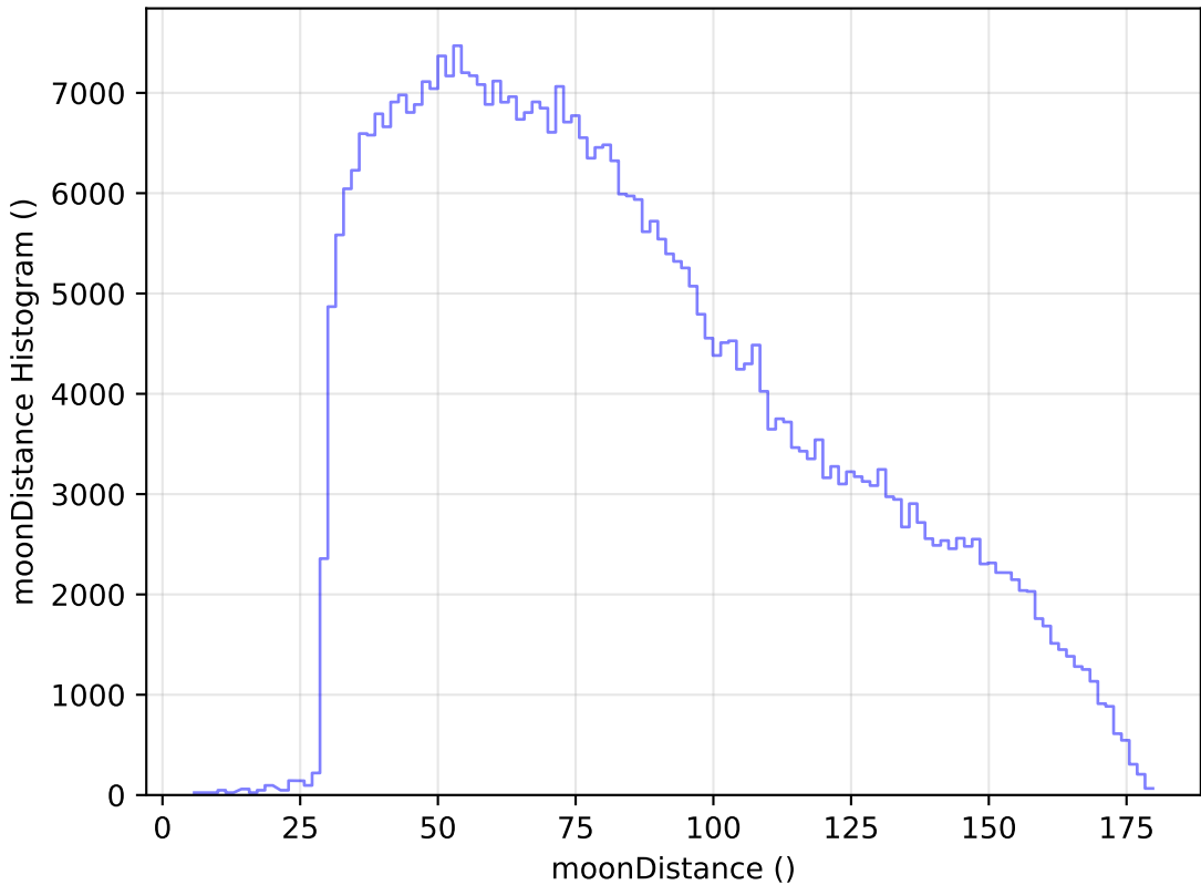
weather_cloudso4v3.4_10yrs WFD z band: moonDistance Histogram
