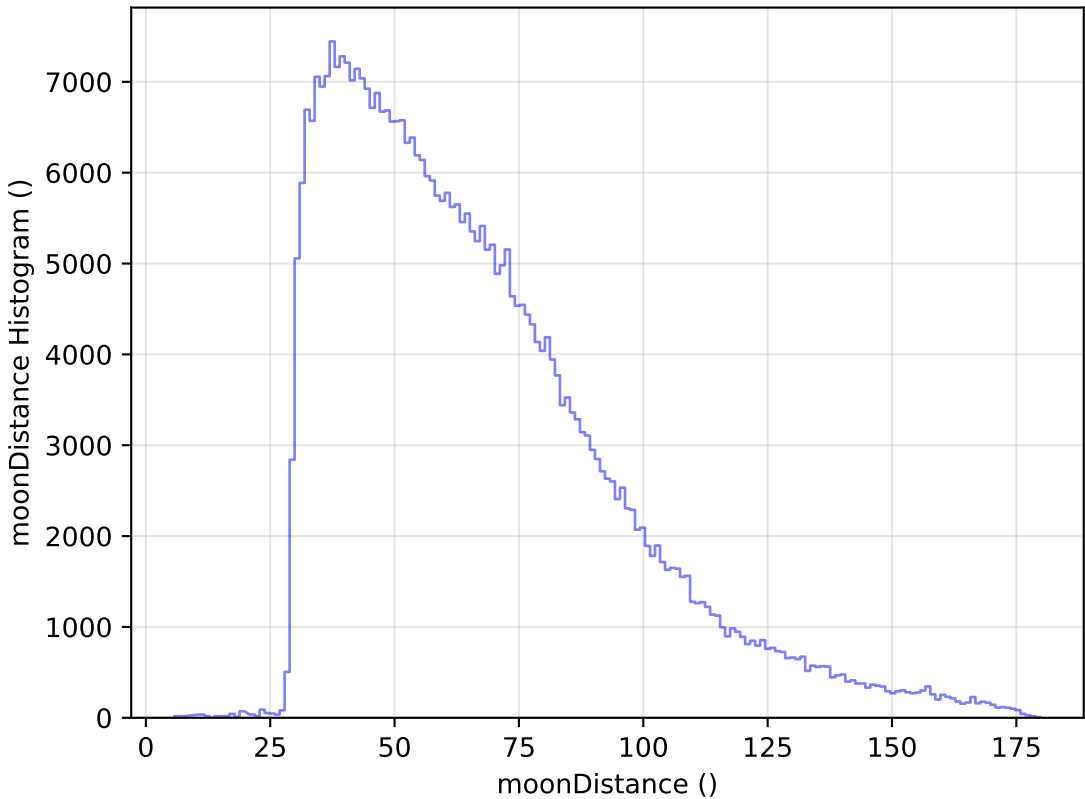
weather_cloudso4v3.4_10yrs WFD y band: moonDistance Histogram
