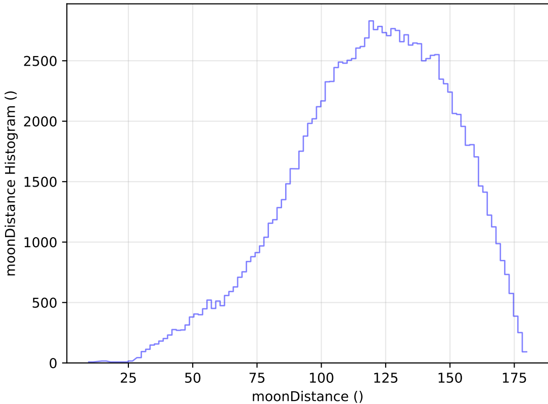
weather_cloudso4v3.4_10yrs WFD u band: moonDistance Histogram
