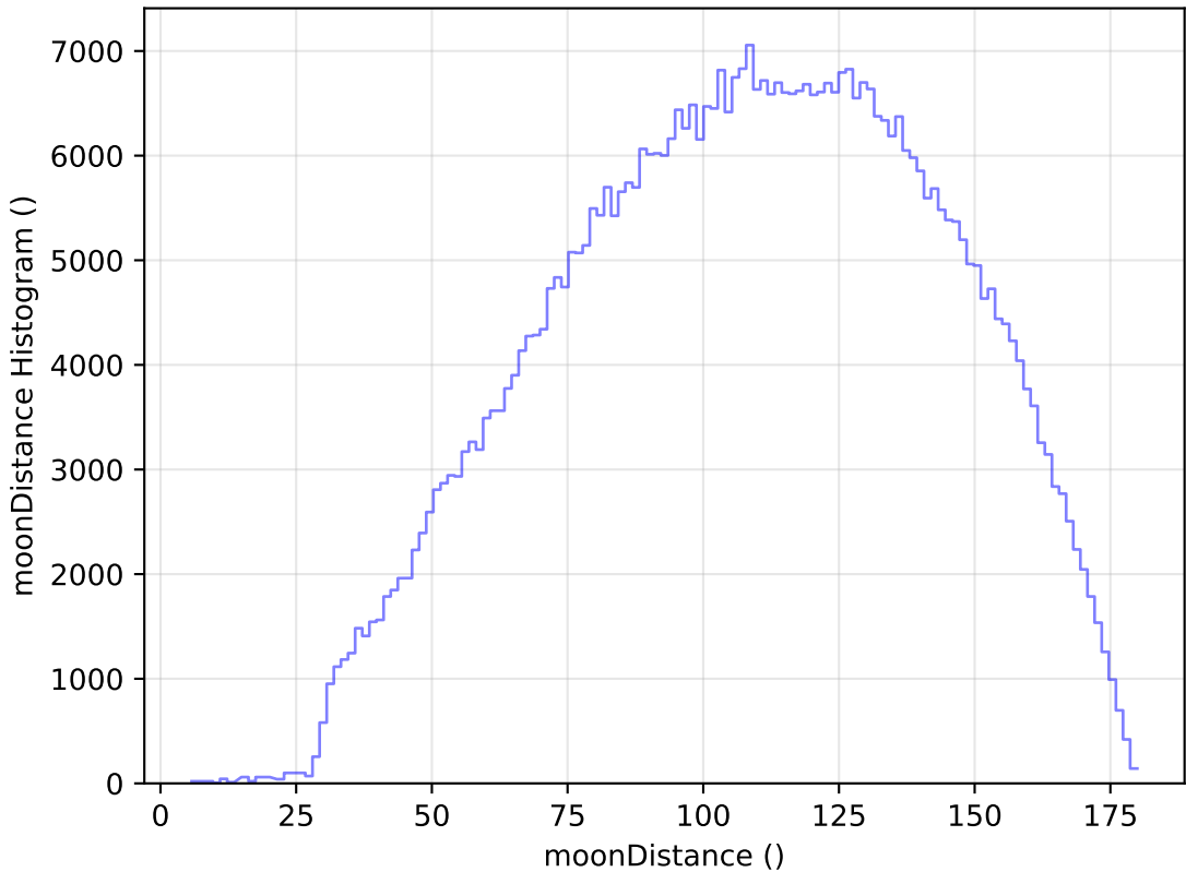
weather_cloudso4v3.4_10yrs WFD r band: moonDistance Histogram
