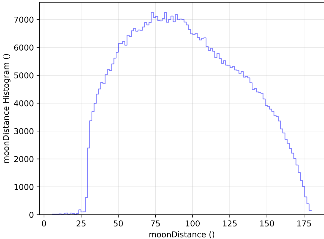
weather_cloudso4v3.4_10yrs WFD i band: moonDistance Histogram
