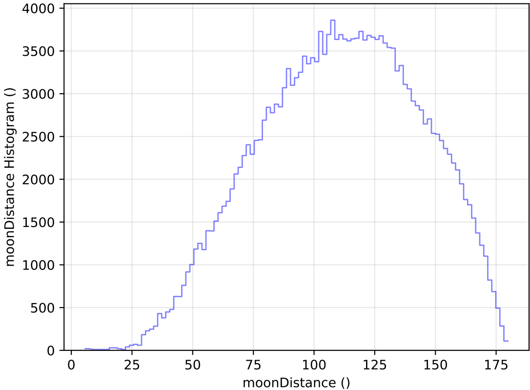
weather_cloudso4v3.4_10yrs WFD g band: moonDistance Histogram
