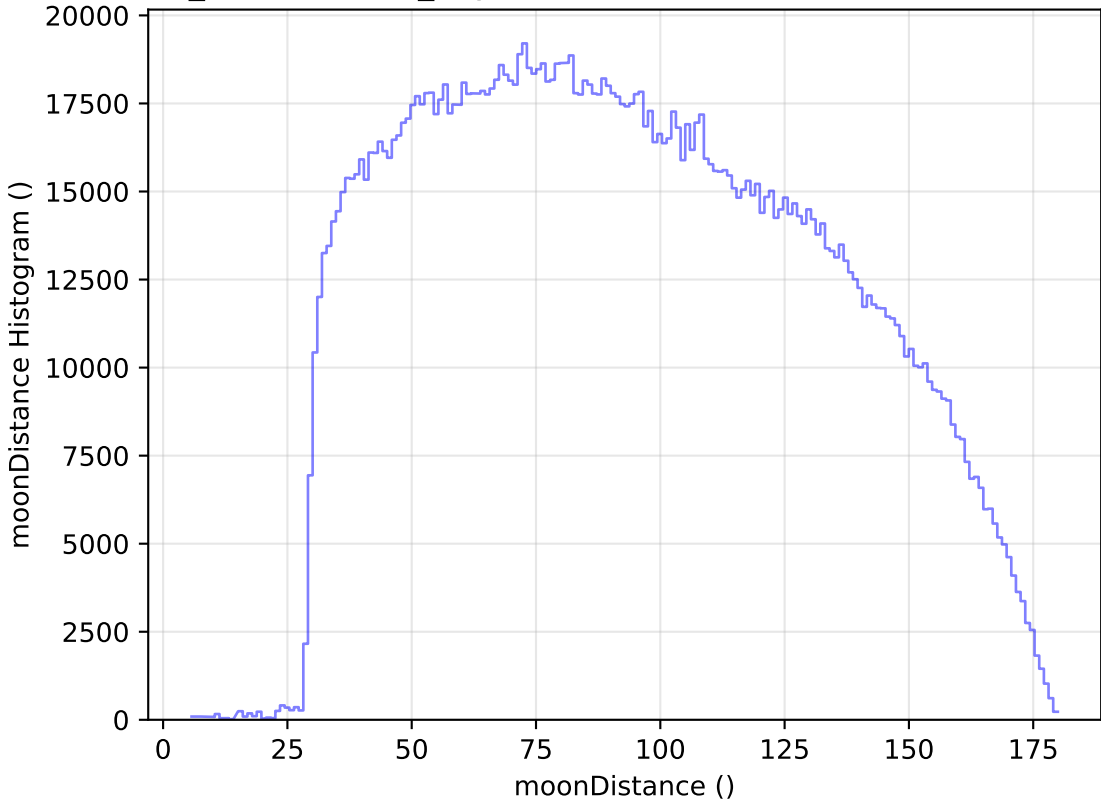
weather_cloudso4v3.4_10yrs WFD all bands: moonDistance Histogram
