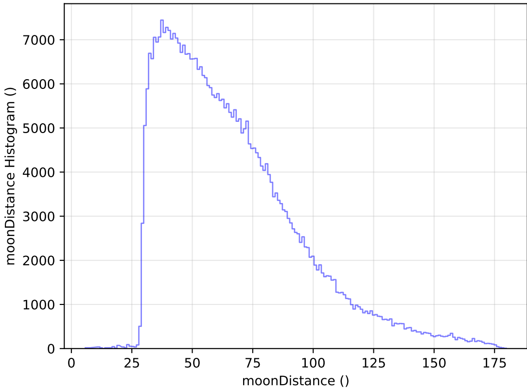
weather_cloudso4v3.4_10yrs All sky y band: moonDistance Histogram
