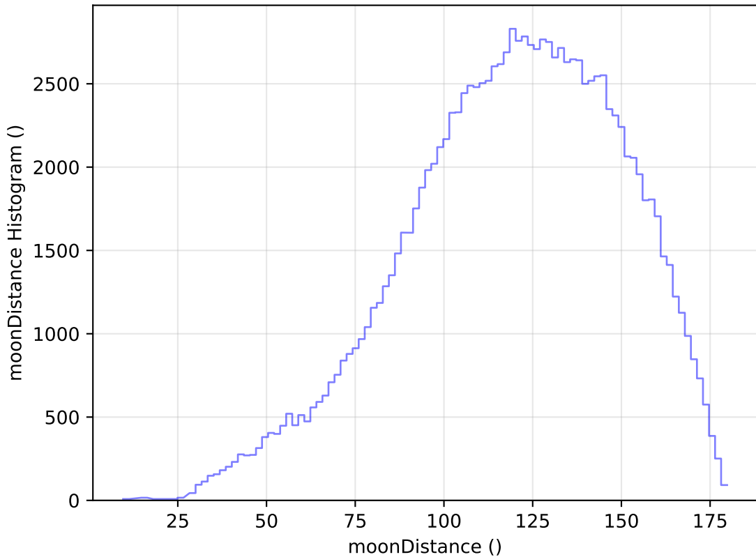
weather_cloudso4v3.4_10yrs All sky u band: moonDistance Histogram
