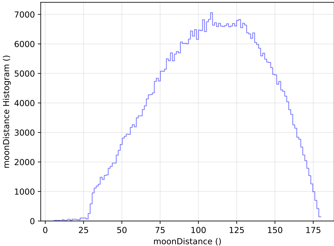
weather_cloudso4v3.4_10yrs All sky r band: moonDistance Histogram
