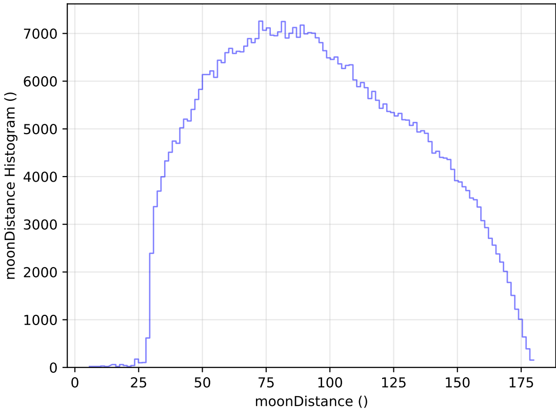
weather_cloudso4v3.4_10yrs All sky i band: moonDistance Histogram
