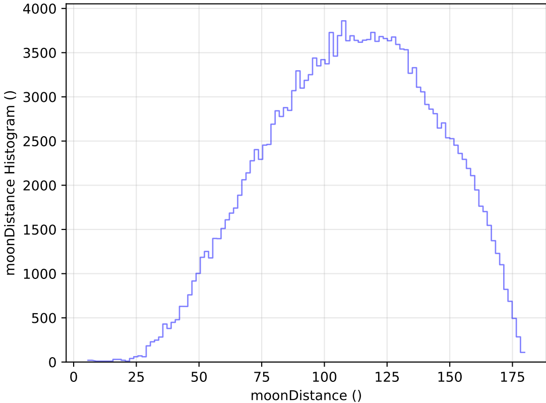
weather_cloudso4v3.4_10yrs All sky g band: moonDistance Histogram
