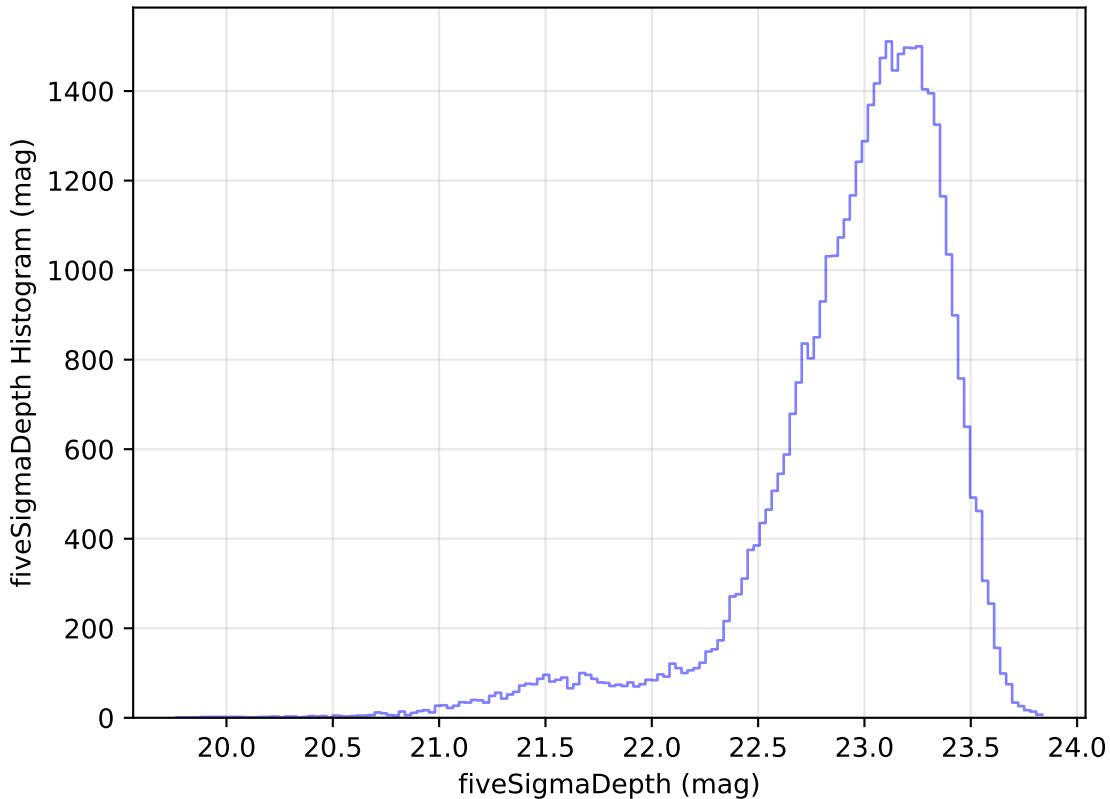
weather_cloudso4v3.4_10yrs Yr 1 z band: fiveSigmaDepth Histogram
