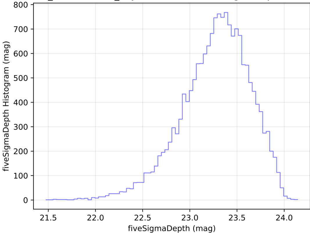
weather_cloudso4v3.4_10yrs Yr 1 u band: fiveSigmaDepth Histogram
