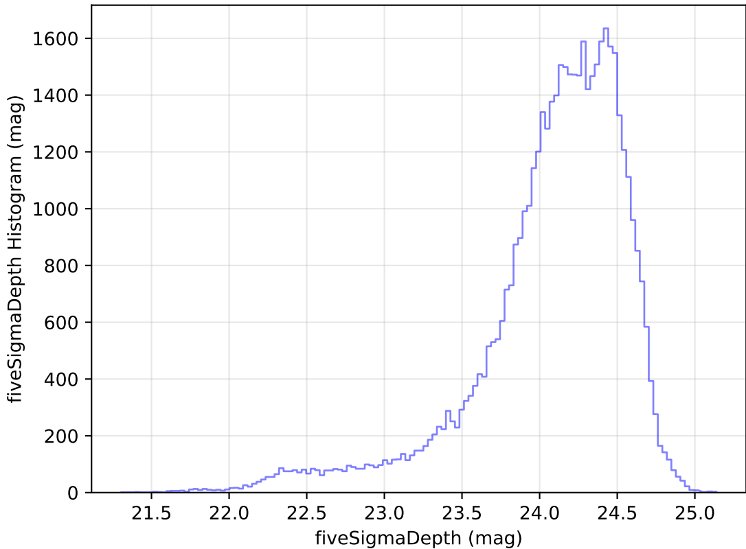
weather_cloudso4v3.4_10yrs Yr 1 r band: fiveSigmaDepth Histogram
