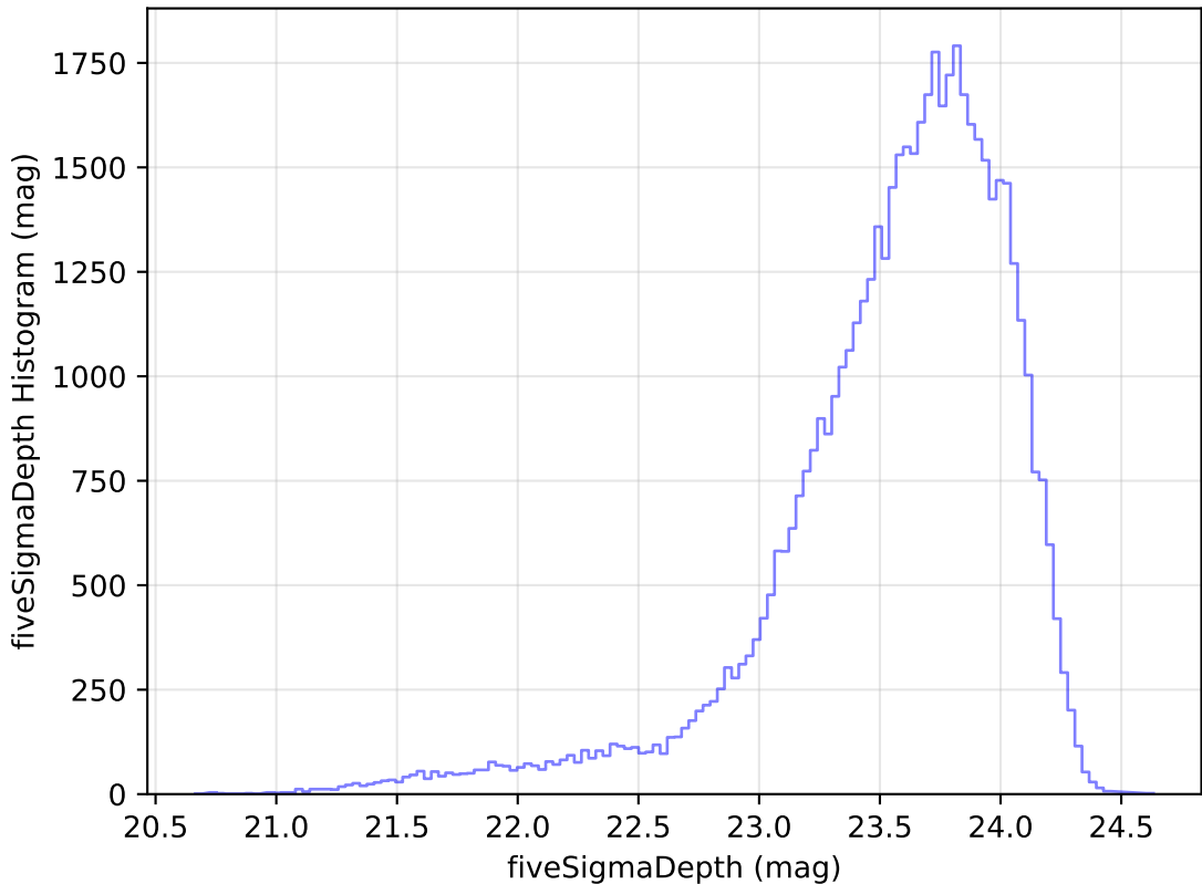
weather_cloudso4v3.4_10yrs Yr 1 i band: fiveSigmaDepth Histogram
