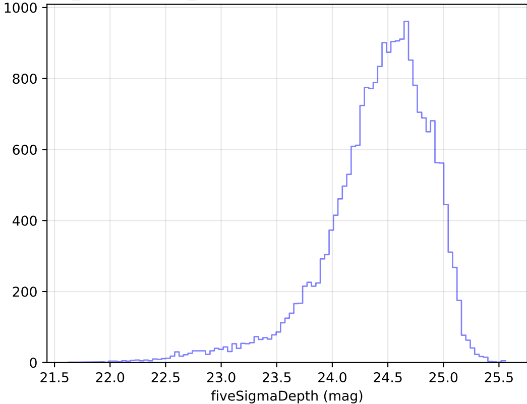
weather_cloudso4v3.4_10yrs Yr 1 g band: fiveSigmaDepth Histogram
