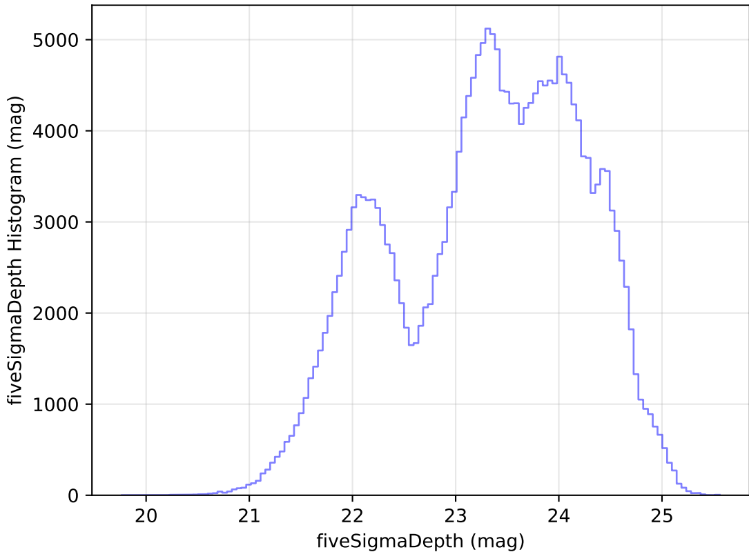
weather_cloudso4v3.4_10yrs Yr 1 all bands: fiveSigmaDepth Histogram
