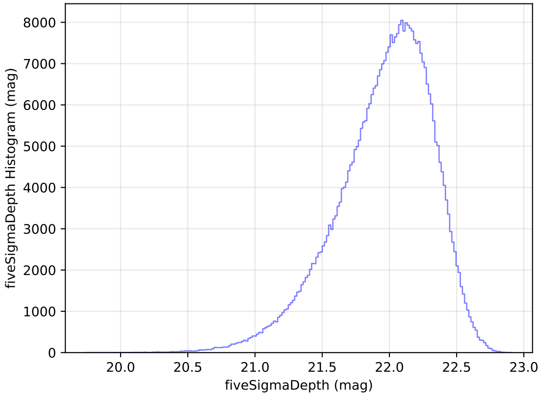
weather_cloudso4v3.4_10yrs WFD y band: fiveSigmaDepth Histogram
