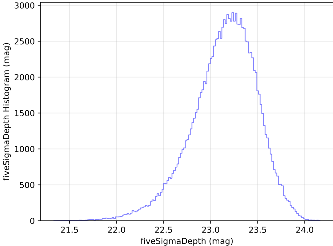
weather_cloudso4v3.4_10yrs WFD u band: fiveSigmaDepth Histogram
