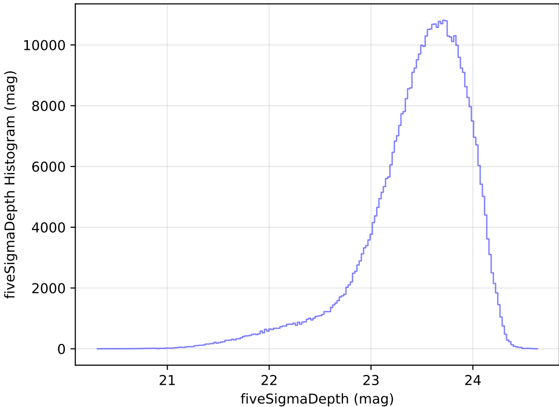
weather_cloudso4v3.4_10yrs WFD i band: fiveSigmaDepth Histogram
