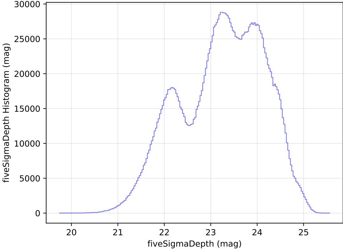
weather_cloudso4v3.4_10yrs WFD all bands: fiveSigmaDepth Histogram
